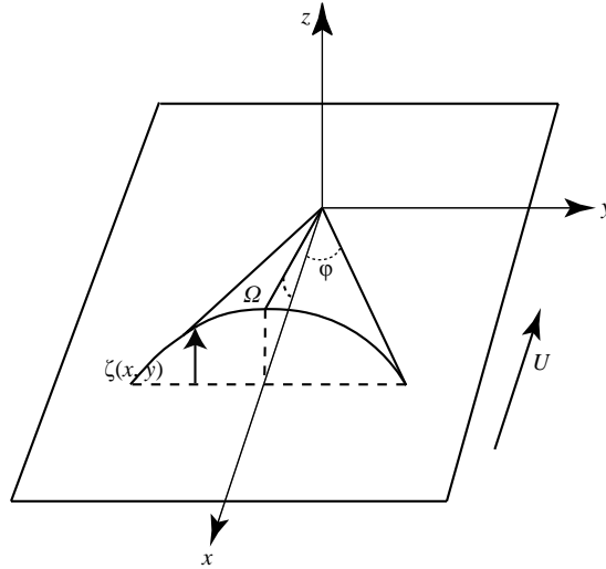
FIGURE 19. Diagram of the rear of a drop on a plate moving upwards at the velocity U such that the drop is in the corner regime. The tail is assumed to be a corner with the opening half-angles \phi and \Omega . \zeta represents the height of the the drop for a given x and y .
